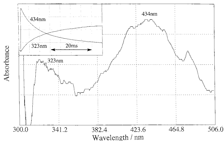
Figure 1. Absorption spectrum of the transient products formed during the irradiation of 3-noradamantyl(phenyl)diazomethane ( 1 ) in degassed benzene recorded 100 \mu s after excitation. Inset shows oscillogram traces monitored at 323 and 434 nm
