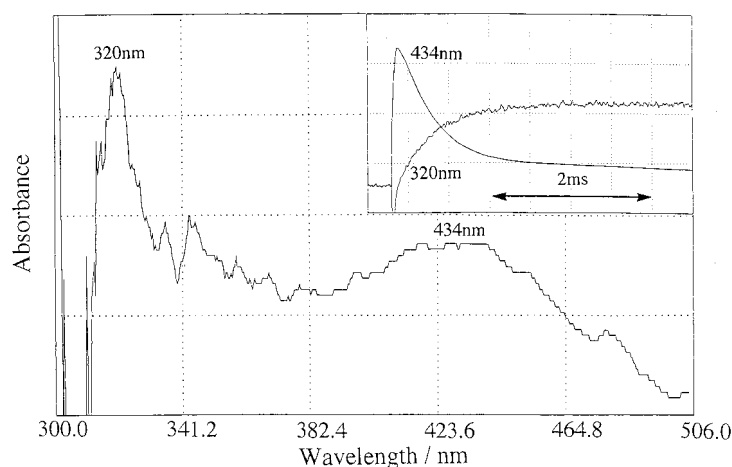
Figure 2. Absorption spectrum of the transient products formed during the irradiation of 1 in degassed benzene containing \text{Bu}_3\text{SnH} ( 3.72 \times 10^{-2} \text{ M} ) recorded 20 \mu s after excitation. Inset shows oscillogram traces monitored at 320 and 434 nm
